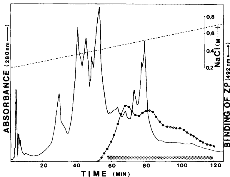
Fig.1. Cation exchange HPLC of ZP-binding proteins. ZP-binding proteins were subjected to a TSK gel SP-5PW and eluted by a gradient elution of 0.2-1M NaCl. The effluents were examined for ZP-binding by the solid-phase binding assay.
